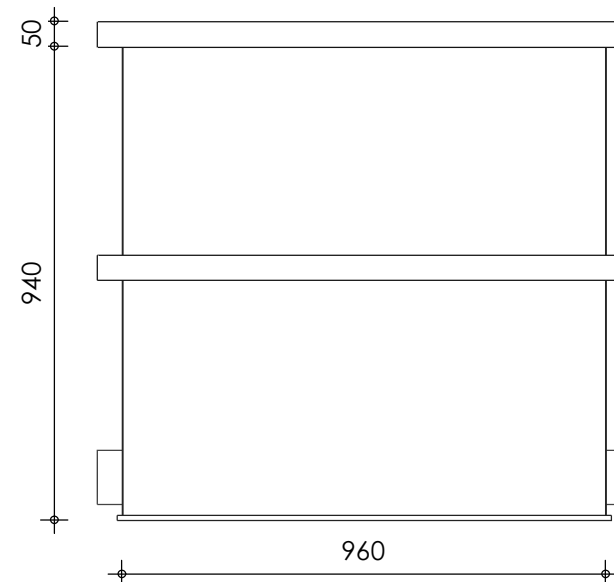
Right-side view
