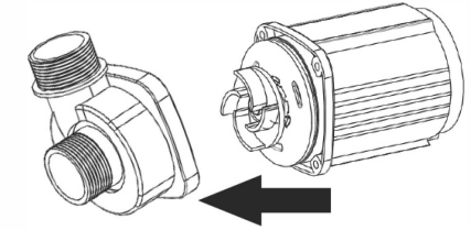
3. Pull pumphouse away from the body
